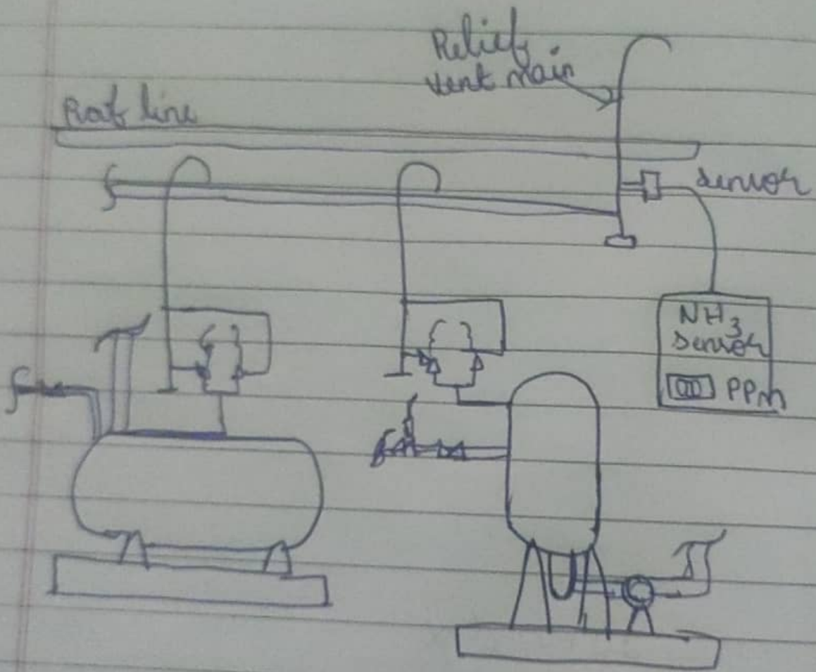
Typical installation of single gas phase ammonia detector in safety relief vent main
