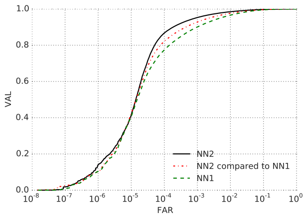
Figure 8. Harmonic Embedding Compatibility. These ROCs show the compatibility of the harmonic embeddings of NN2 to the embeddings of NN1. NN2 is an improved model that performs much better than NN1. When comparing embeddings generated by NN2 to the harmonic ones generated by NN1 we can see the compatibility between the two. In fact, the mixed mode performance is still better than NN1 by itself.
